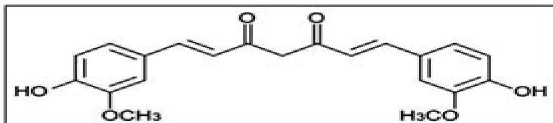
Curcuminoids
