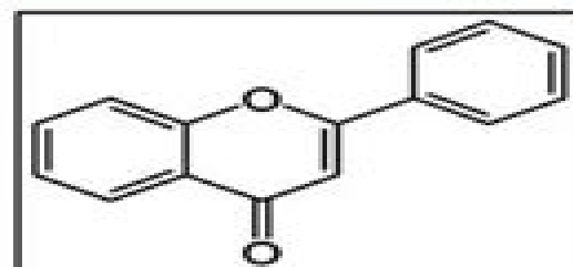
Flavonoids
